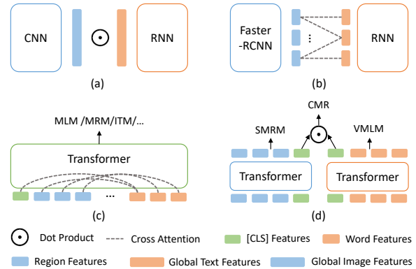
Figure 1: Evolution of Image-Text Retrieval (ITR) paradigm. (a) Early work (Faghri et al., 2017) using dot product to learn the similarity between global image features and global text features. (b) Later study (Lee et al., 2018) applying cross-attention between the features of each region and each word. (c) Pre-trained V+L models (Chen et al., 2020) with deep Transformer. (d) LightningDOT without cross-attention. CMR, SMRM and VMLM refer to different pre-training tasks, which will be introduced later in method section.
